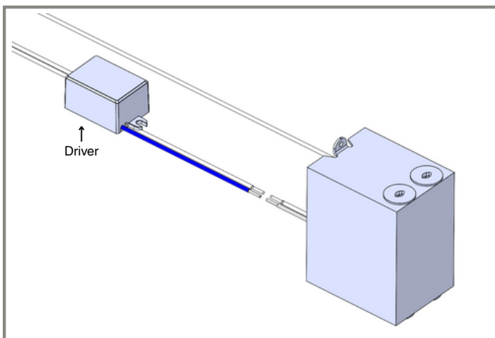
3. Connect the neutral wire from the wall to the input wire (shown as “blue” wire) on the driver.
